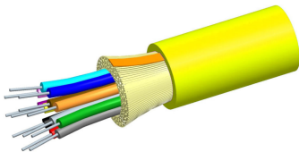
TeraSPEED® Low Smoke Zero Halogen Riser Distribution Cable, 6 fiber single-unit, singlemode, yellow
